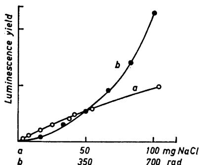
Fig. 7. The effect on the luminescence observed when the concentration of e_{\text{aq}}^- ( = \text{Cl}\cdot ) is increased either by a) increasing the amount of irradiated NaCl dissolved at a constant dose (350 rad), or by b) increasing the dose using a constant amount of NaCl (50 mg). The same results are obtained independent of if 0.5, 1, or 2 ml fluorescein solution is injected.
